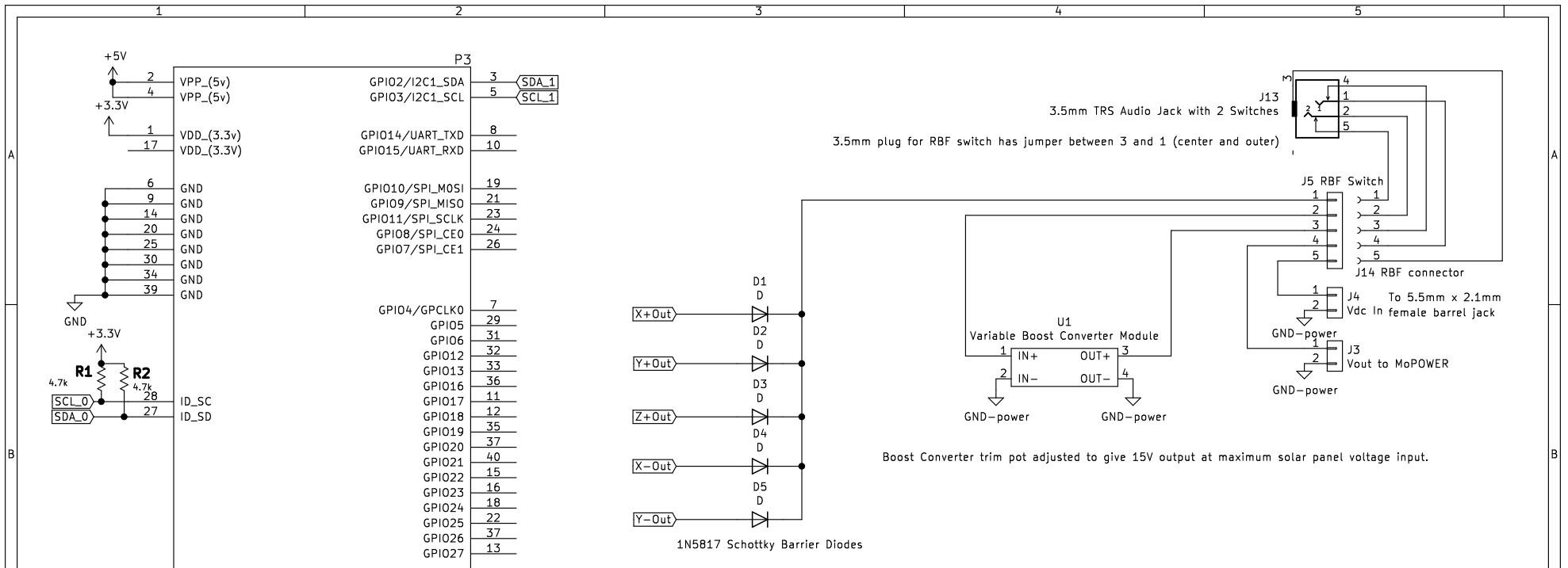
Raspberry Pi GPIO Connector Male Extra Long (19mm) 20x2 Header Pins
